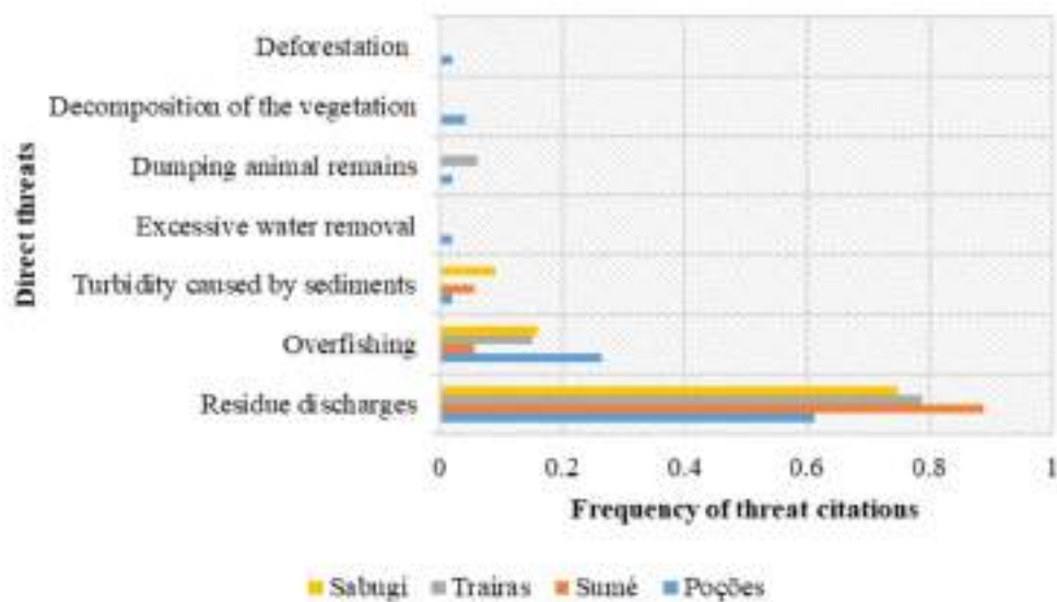
Figure 2. Main threats to the studied reservoirs indicated by the local population. Traíras and Sabugí Reservoirs, Piranhas-Assú river watershed; Sumé and Poçoês Reservoirs, Paraíba River watershed, Brazil.
