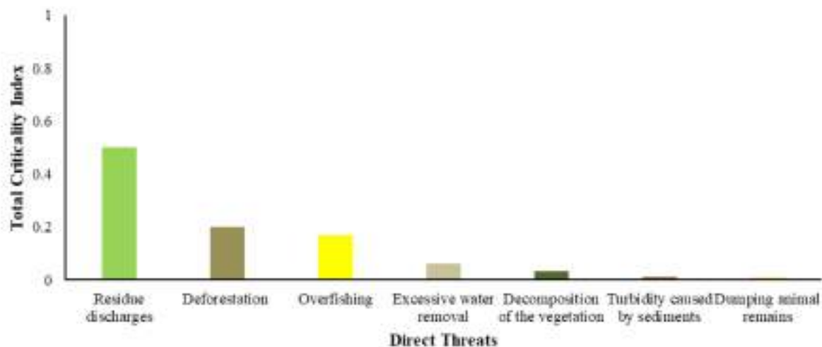
Figure 3. Criticality Index of the threats on the researched reservoirs. Traíras and Sabugi reservoirs, Piranhas-Assu river watershed; Sumé and Poções reservoirs, Paraíba river watershed, Brazil.
